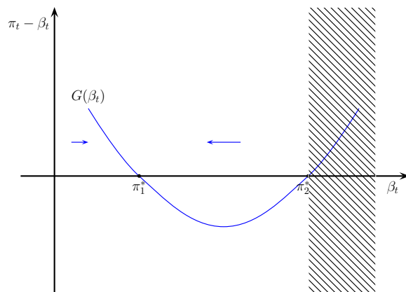
FIGURE 2. Adaptive dynamics and the “escape event”.
